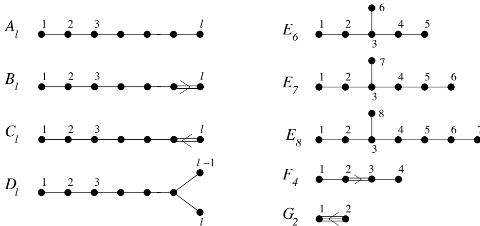
Figure 3.2: Dynkin diagrams
