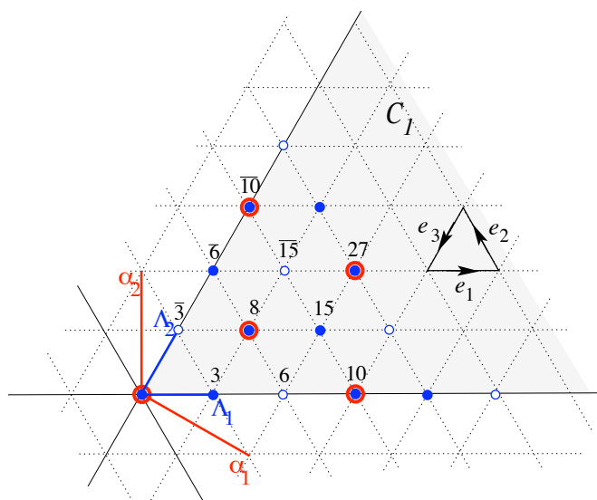
Figure 3.4: Weights of su(3) . Only the first Weyl chamber \mathcal{C}_1 has been detailed, with some highest weights. The weights of triality 0 (forming the root lattice) are represented by a wide disk, those of triality 1, resp. 2, by a full, resp. open disk.
