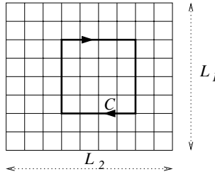
Figure 5.3: Square lattice in 2 d
