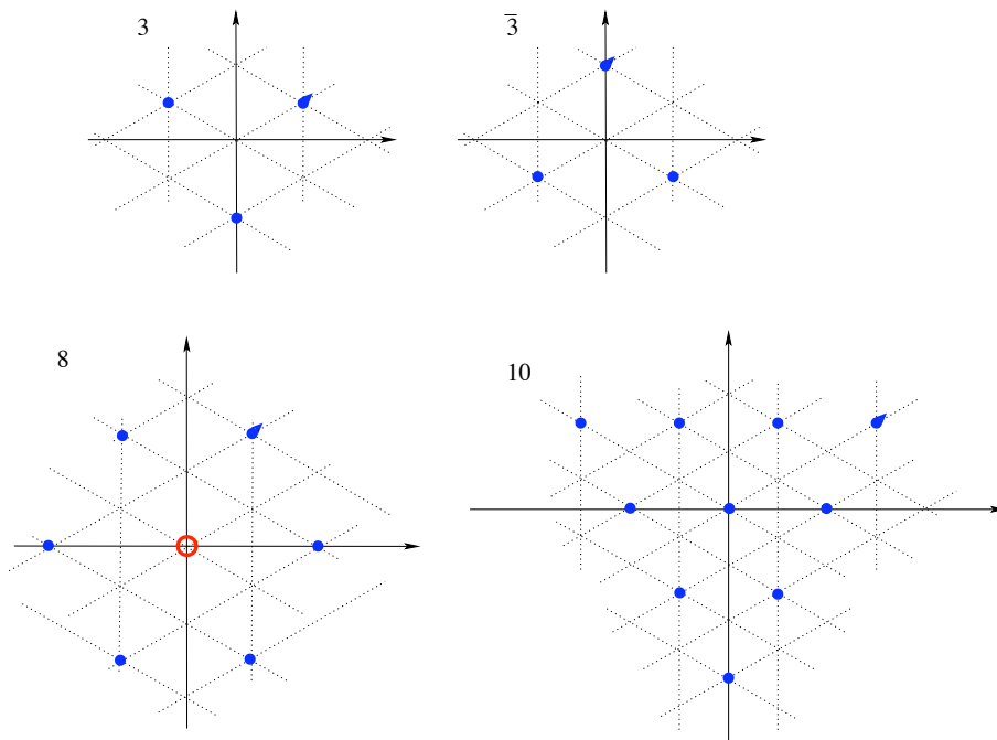
Figure 3.5: The weight diagrams of low lying representations of su(3) , denoted by their dimension. Note that a rotation of 30^\circ of the weight lattice has been performed with respect to the previous figure. In each representation, the highest weight is marked by a small indentation. The small dots are weights of multiplicity 1, the wider open dot has multiplicity 2.
